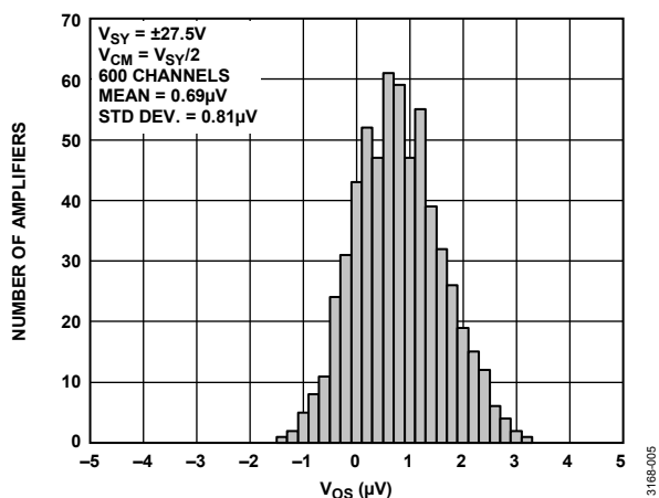
Figure 6. Input Offset Voltage Distribution, V_{SV} = \pm 27.5\text{ V}
