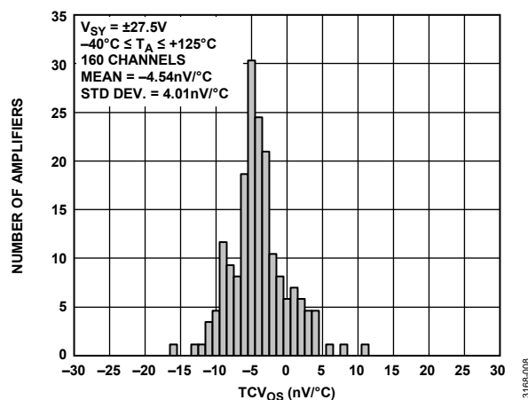
Figure 9. Input Offset Voltage Drift Distribution, V_{SV} = \pm 27.5\text{ V}
