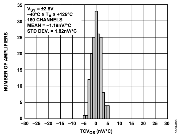
Figure 7. Input Offset Voltage Drift Distribution, V_{SV} = \pm 2.5\text{ V}
