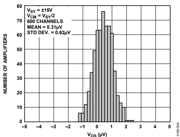
Figure 5. Input Offset Voltage Distribution, V_{SV} = \pm 15\text{ V}
