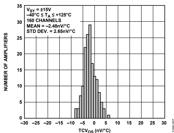
Figure 8. Input Offset Voltage Drift Distribution, V_{SV} = \pm 15\text{ V}
