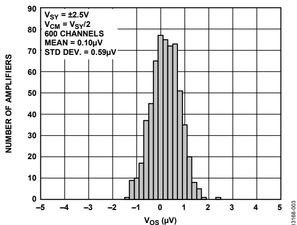
Figure 4. Input Offset Voltage Distribution, V_{SV} = \pm 2.5\text{ V}
