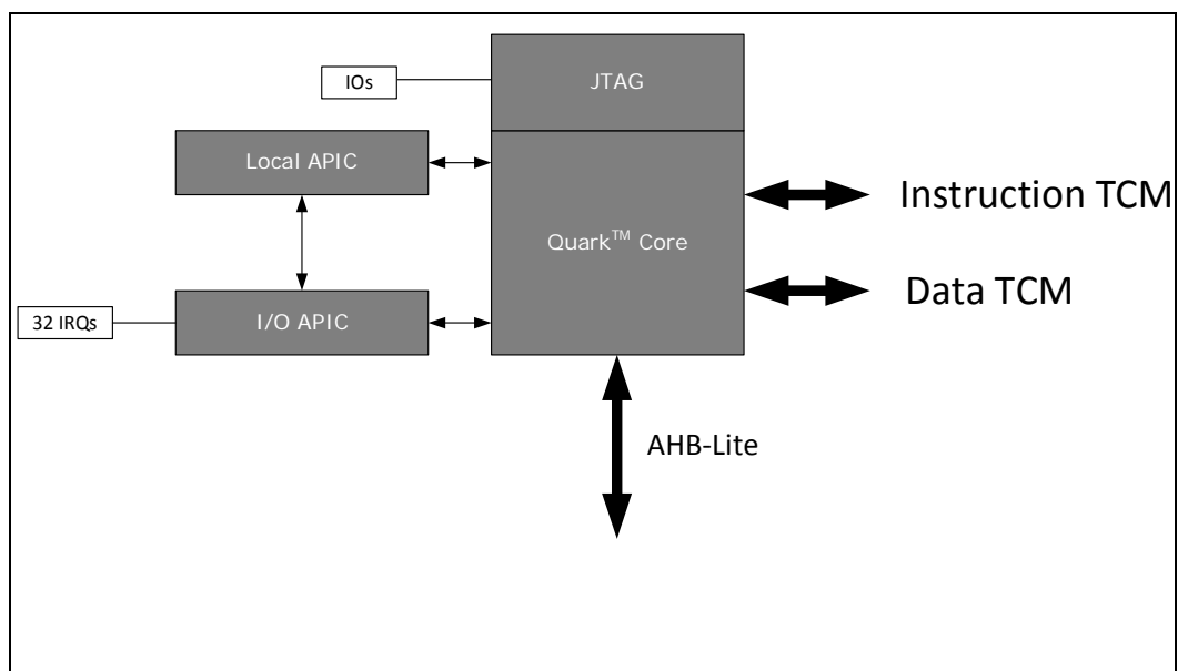
Figure 8. Processor Core
