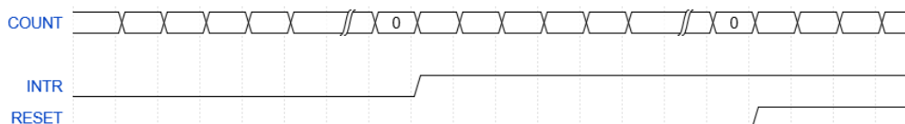
Figure 15. WDT Behaviour for Response Mode of 1
