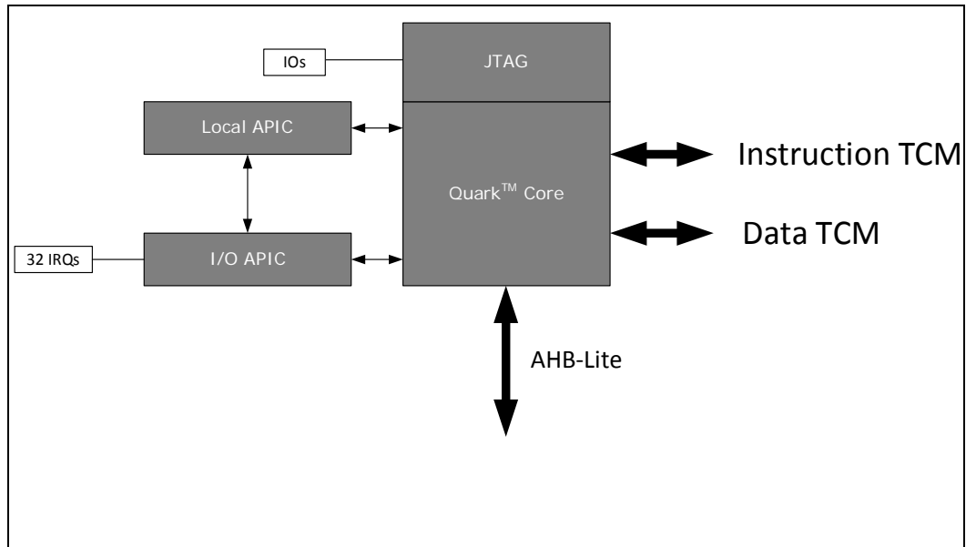
Figure 8. Processor Core
