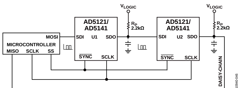
Figure 40. Daisy-Chain Configuration
