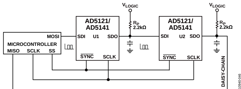
Figure 40. Daisy-Chain Configuration
