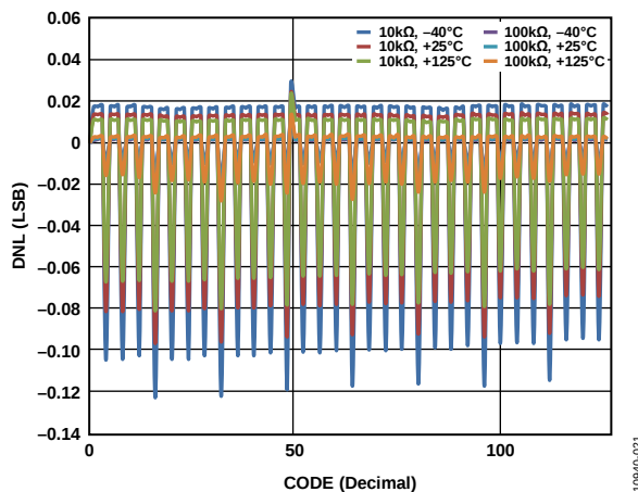
Figure 18. DNL vs. Code (AD5121)
