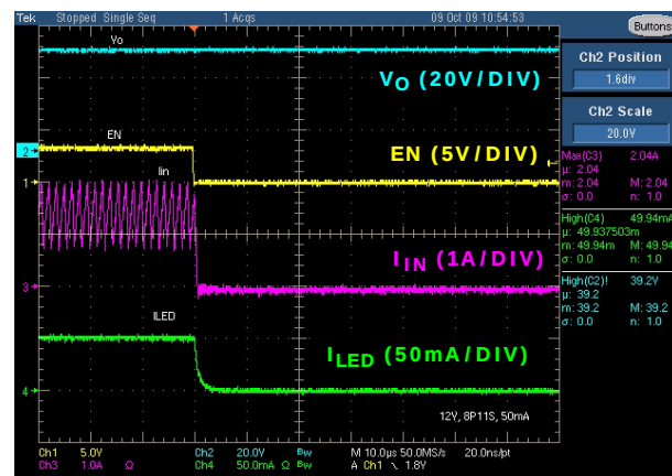
FIGURE 24. DISABLE PROFILE
