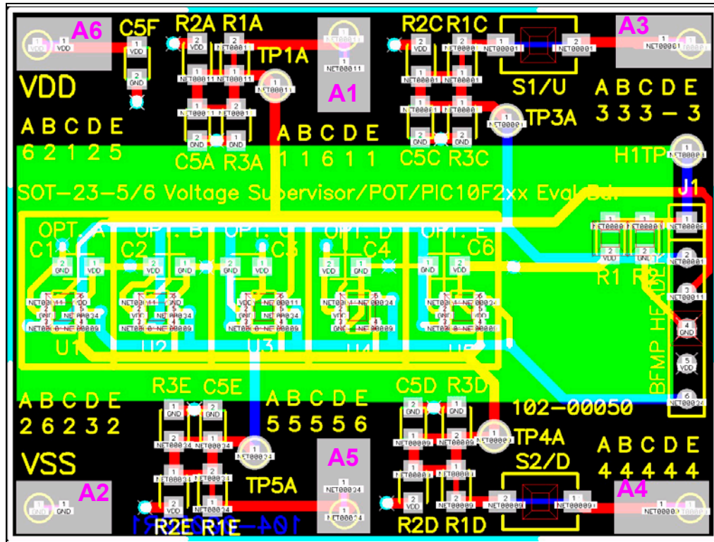
FIGURE 2-2: Voltage Supervisor SOT-23-5/6 Evaluation Board Layout with added "Pad Names".
