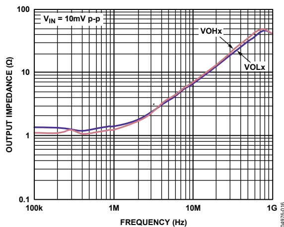
Figure 17. Output Resistance at VOHx and VOLx Pins vs. Frequency
