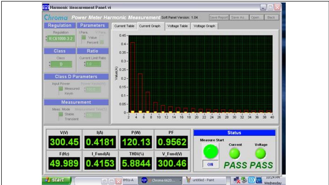
Figure 17 Input Current Harmonic Spectrum at Full Load and V_{IN} = 300\text{ VAC}
