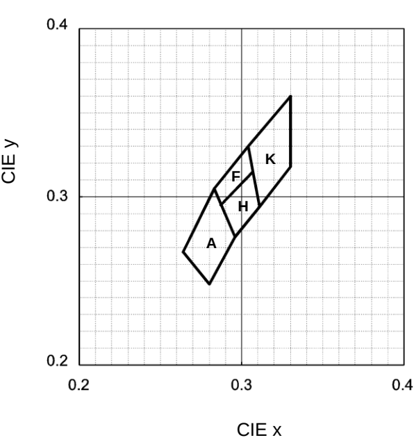
[Chromaticity Coordinates] (Ta=25°C, If=5mA)
