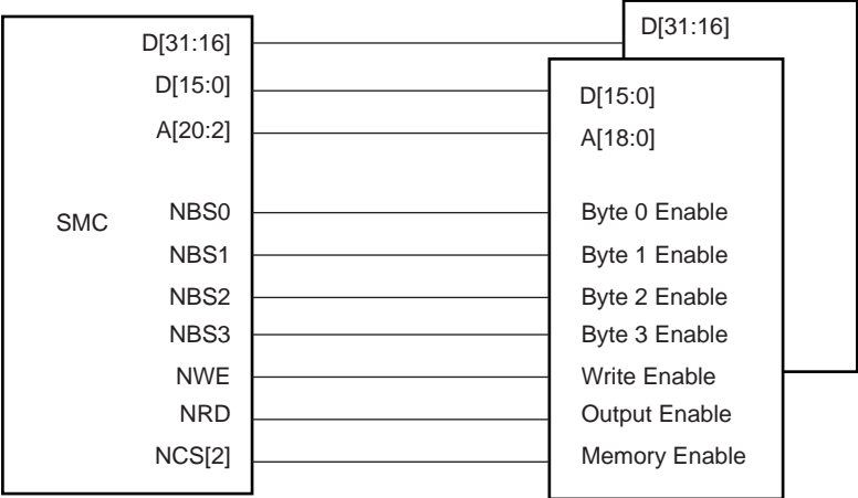
Figure 20-5. Memory Connection for a 32-bit Data Bus
