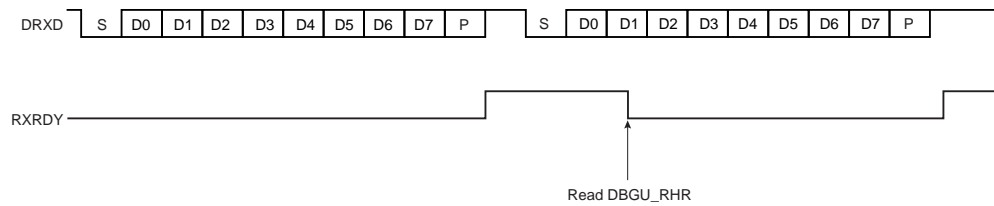
Figure 27-6. Receiver Ready
