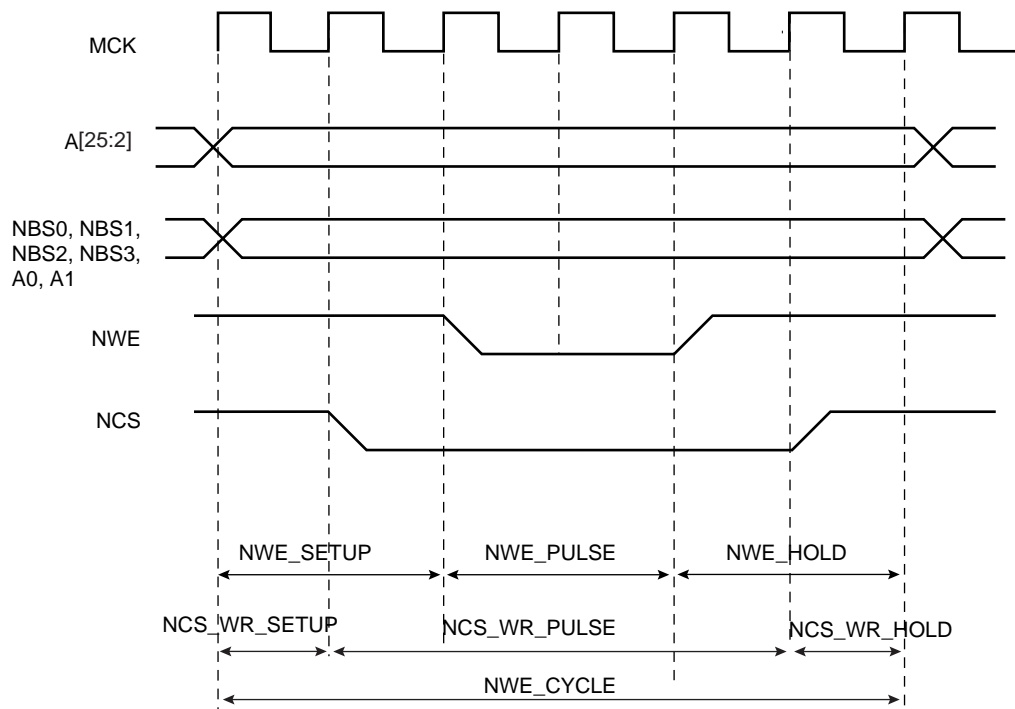
Figure 20-12. Write Cycle
