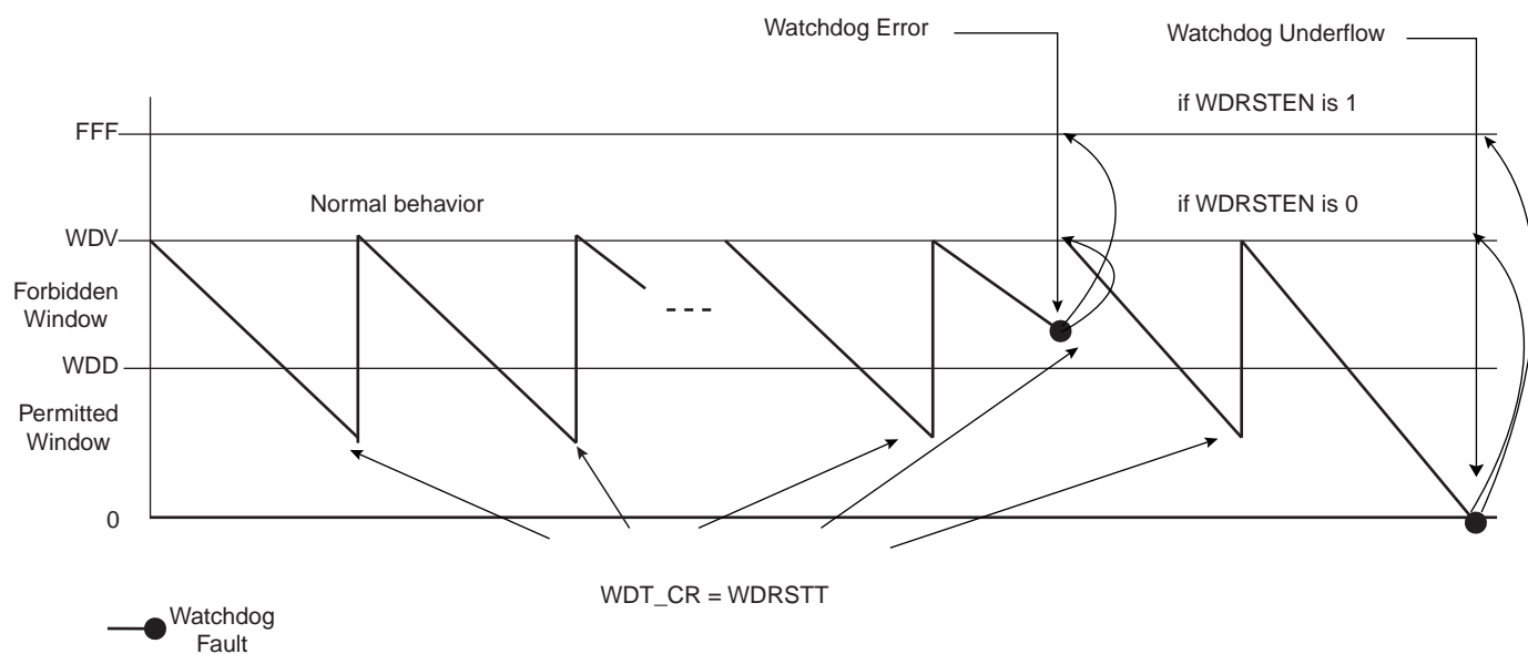
Figure 25-2. Watchdog Behavior
