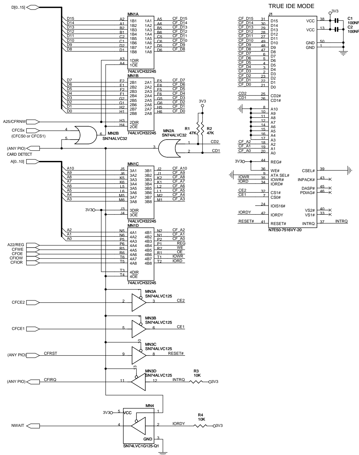
Figure 19-9. Hardware Configuration
