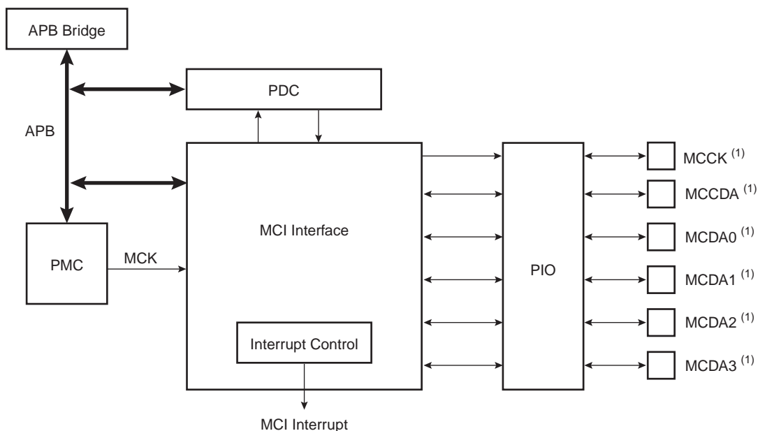
Figure 34-1. Block Diagram
