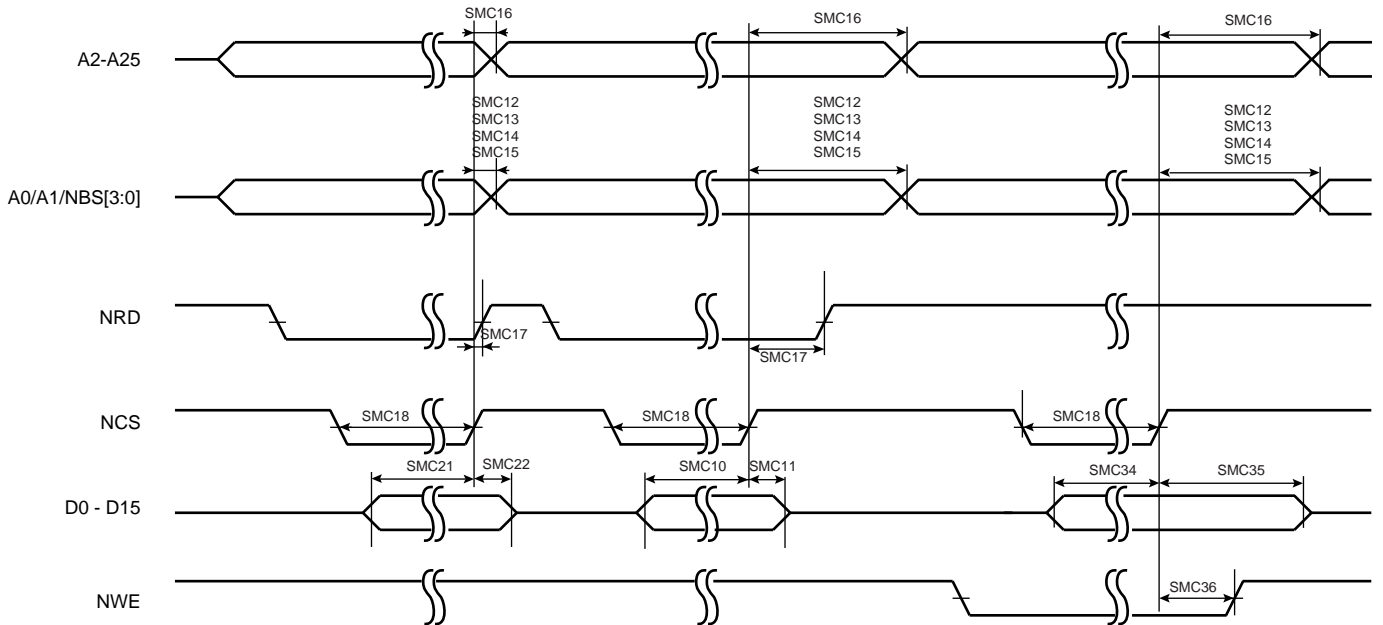
Figure 38-4. SMC NCS Controlled Access
