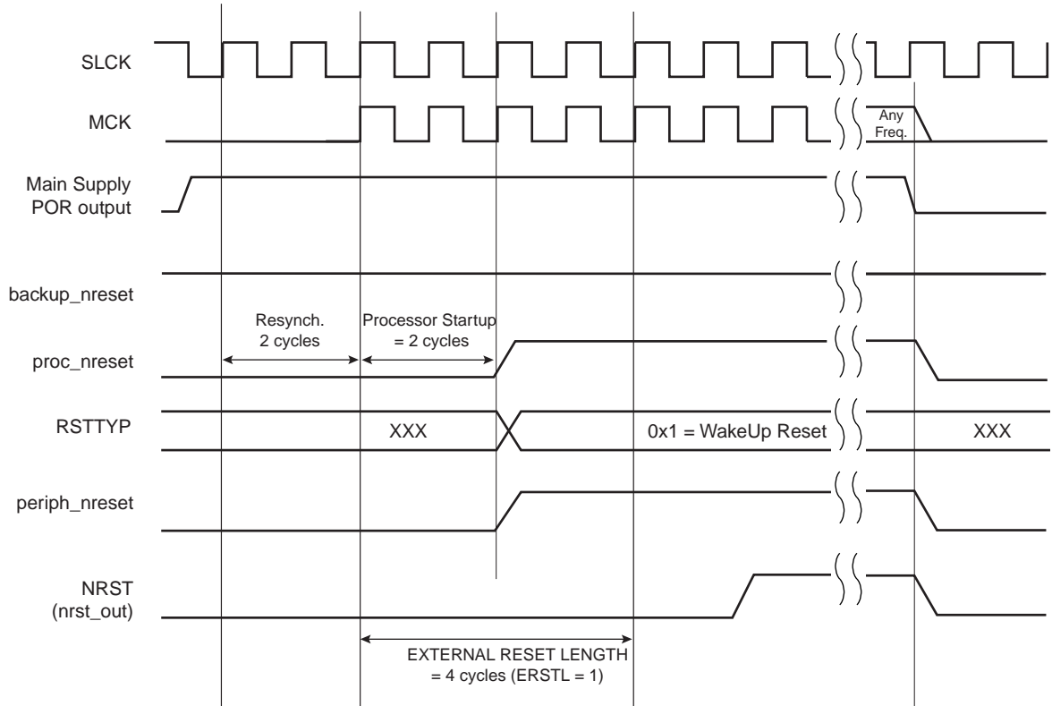
Figure 13-5. Wakeup State
