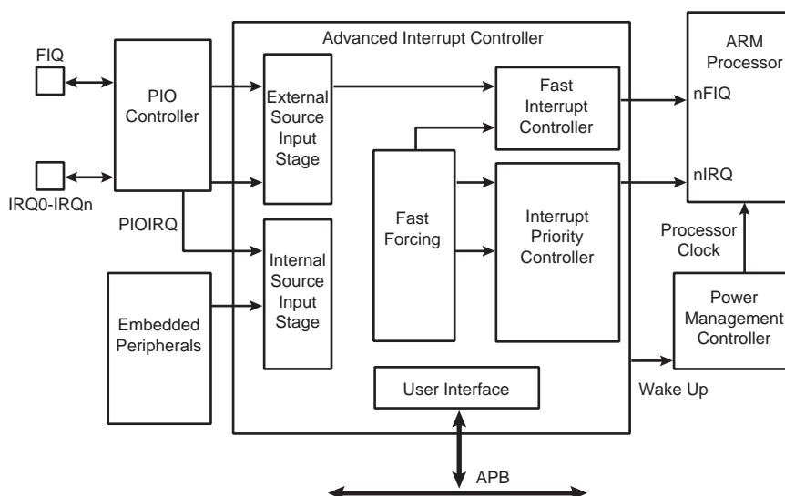
Figure 26-3. AIC Detailed Block Diagram
