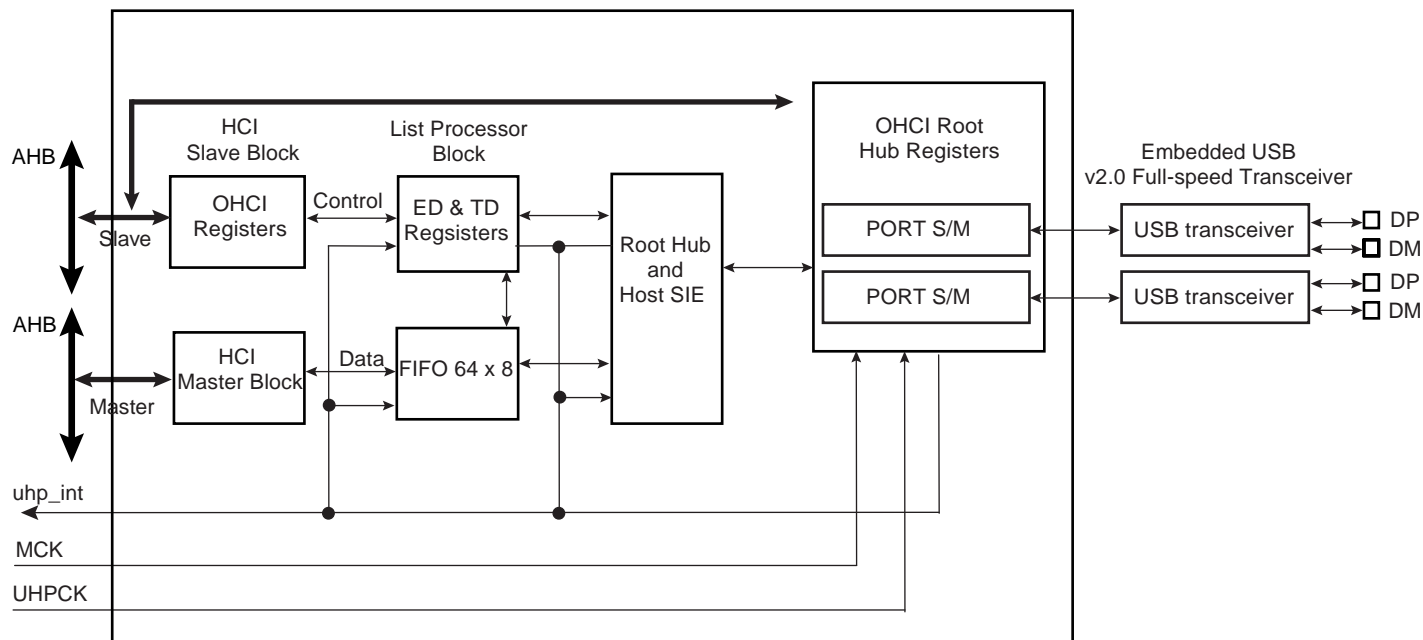
Figure 35-1. Block Diagram
