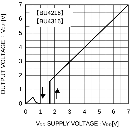
Fig.6 I/O Characteristics
