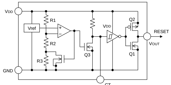
Fig.16 (BU43xx type Internal Block Diagram)
