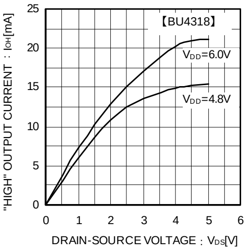
Fig.5 "High" Output Current
