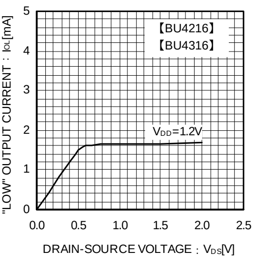
Fig.4 "LOW" Output Current
