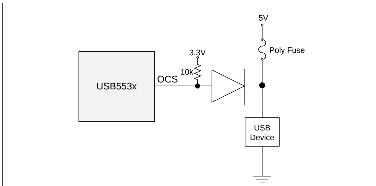
FIGURE 4-13: POLY-FUSE IMPLEMENTATION
