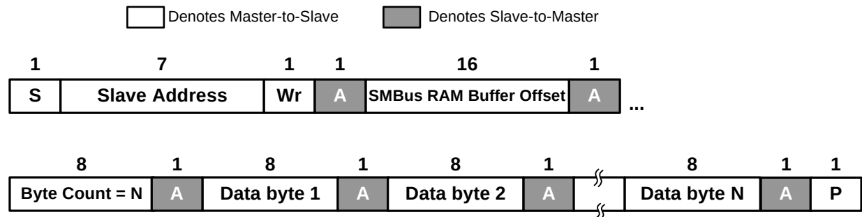
FIGURE 5-4: BLOCK WRITE
