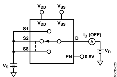
Figure 23. I_D (Off)
