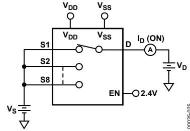
Figure 24. I_D (On)
