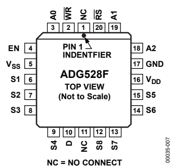
Figure 7. ADG528F Pin Configuration PLCC
