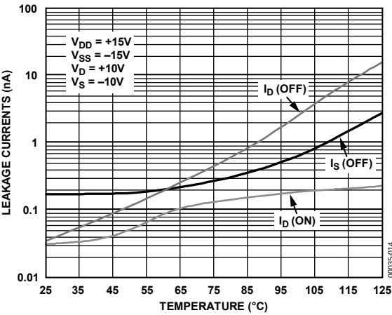
Figure 14. Leakage Currents as a Function of Temperature
