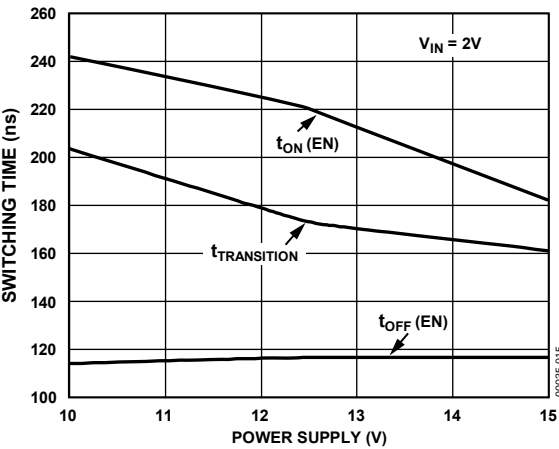
Figure 15. Switching Time vs. Power Supply
