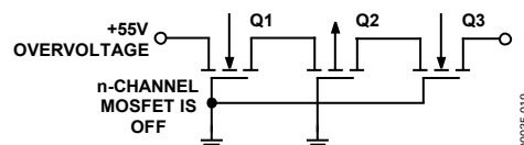
Figure 19. +55\text{ V} Overvoltage with Power Off
