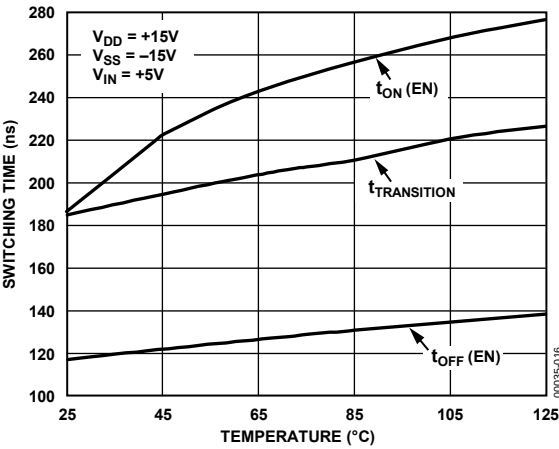
Figure 16. Switching Time vs. Temperature
