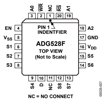
Figure 7. ADG528F Pin Configuration PLCC
