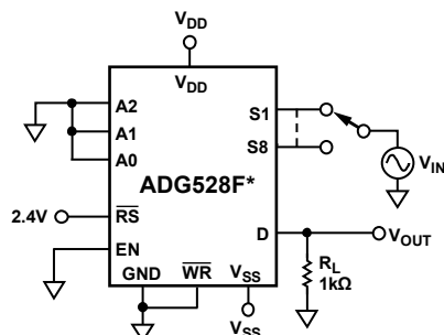
Figure 33. Off Isolation
