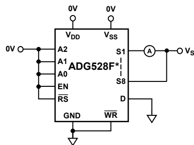
Figure 26. Input Leakage Current (with Power Supplies Off)
