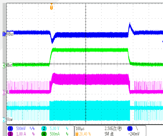
Load Transient
