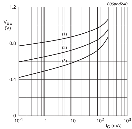
V_{CE} = 6 \text{ V} (1) T_{amb} = -55 \text{ }^\circ\text{C} (2) T_{amb} = 25 \text{ }^\circ\text{C} (3) T_{amb} = 100 \text{ }^\circ\text{C}
