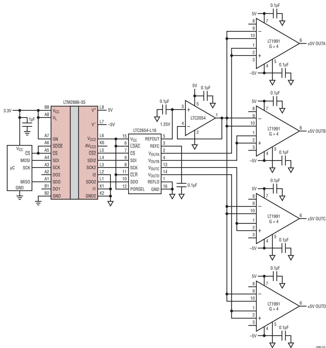
Figure 25. Quad 16-Bit ±5V Output Range DAC
