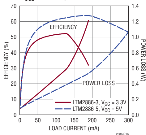
V_{CC2} Efficiency
