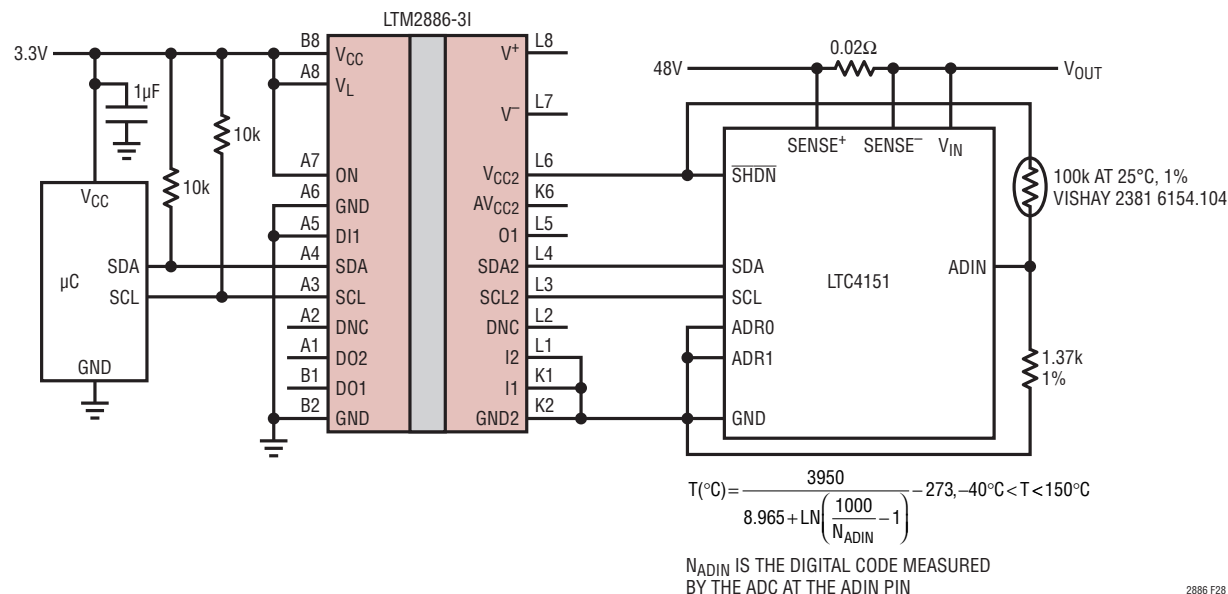
Figure 28. Isolated I²C Voltage, Current and Temperature Power Supply Monitor
