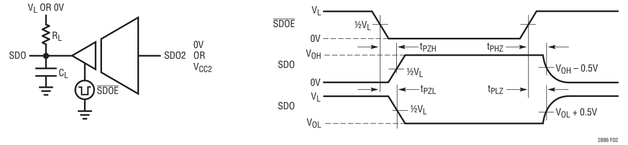
Figure 2. Logic Enable/Disable Time
