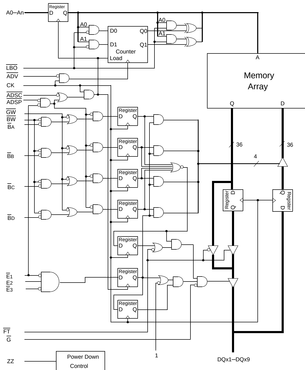
GS88118/32/36C(T/D)-xxxV Block Diagram
