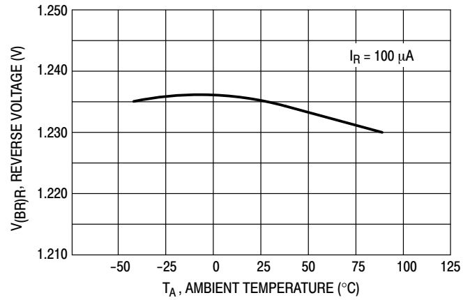
Figure 5. Temperature Drift
