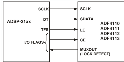
Figure 39. ADSP-21xx to ADF4110 Family Interface
