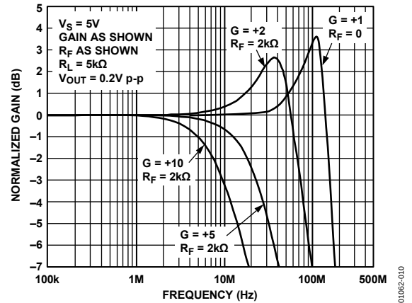
Figure 10. AD8054 Normalized Gain vs. Frequency; V_S = 5V
