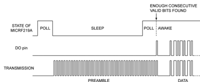
Figure 14. Sufficient Preamble Length
