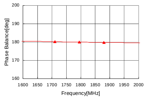
Phase Balance
