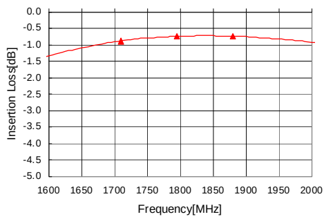
Insertion Loss
