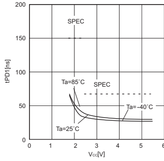
Fig.25 Data output delay time t_{PD1} (CL=100pF)
