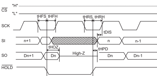
Fig. 5 HOLD timing
