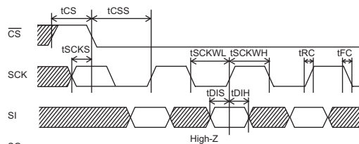
Fig. 3 Input timing
