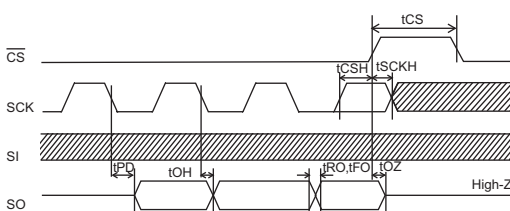
Fig. 4 Input / output timing
