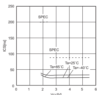
Fig.20 CS high time tCS
