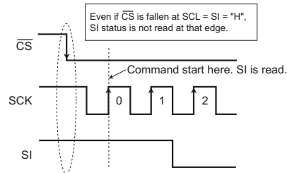
Fig.45 Operating timing
