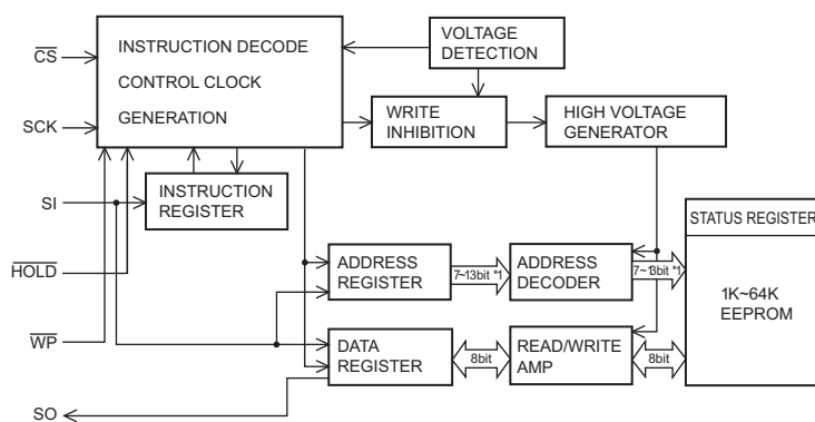
Fig.1 Block diagram
