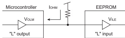
Fig.53 Pull up resistance
