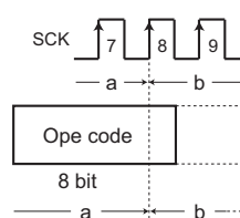
Fig.52 WREN / WRDI cancel valid timing
