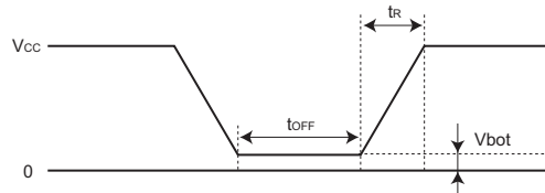
Fig.64 Rise waveform
