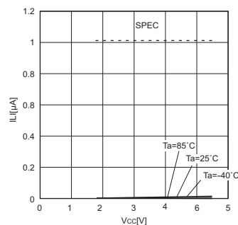
Fig.12 Input leak current I_{IL}(CS,SCK,SI,WP,HOLD)
