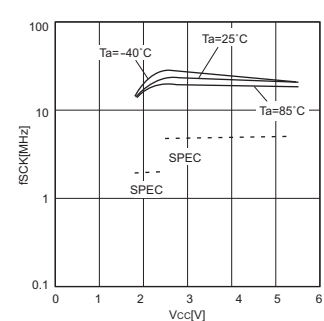
Fig.17 SCK frequency fSCK
