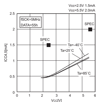
Fig.15 Consumption current at READ operation ICC_{4,5}(READ,WRSR,fSK=5MHz)
