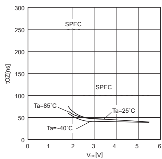
Fig.27 Output disable time t_{OZ}
