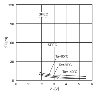
Fig.33 Output fall time
