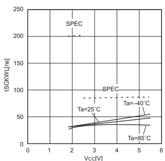
Fig.19 SCK low time tSCKWL
