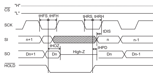
Fig. 5 HOLD timing
