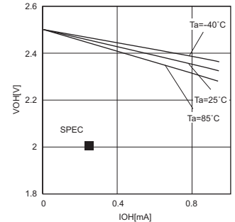
Fig.11 "H" output voltage V_{OH-IOH}(V_{CC}=2.5V)
