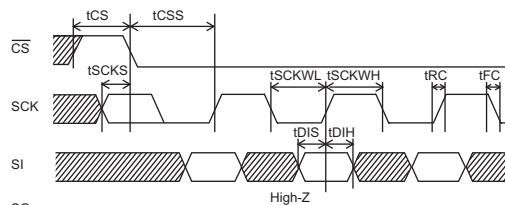
Fig. 3 Input timing
