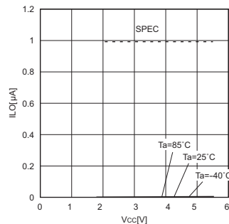
Fig.13 Output leak current I_{LO}(SO)
