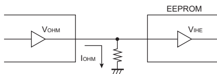
Fig.54 Pull down resistance
