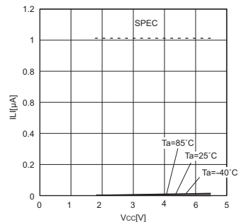
Fig.12 Input leak current I_{IL}(CS,SCK,SI,HOLD)
