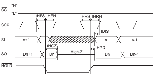
Fig. 5 HOLD timing
