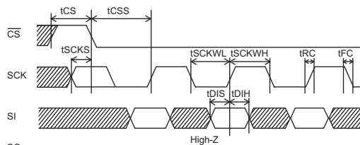
Fig. 3 Input timing
