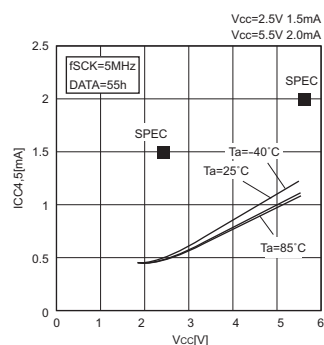
Fig.15 Consumption current at READ operation ICC_{4,5}(READ,WRSR,fSK=5MHz)
