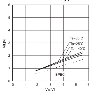
Fig.7 "L" input voltage V_{IL}(C\bar{S}, SCK, SI, \overline{HOLD}, \overline{WP})
