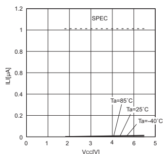
Fig.12 Input leak current I_{IL}(C\bar{S}, SCK, SI, \overline{WP}, \overline{HOLD})
