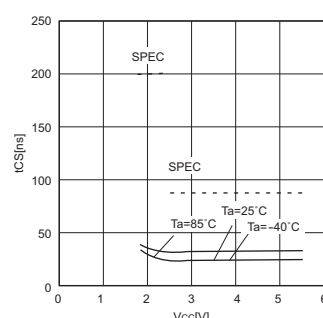
Fig.20 \bar{CS} high time t_{CS}
