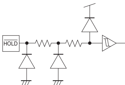
Fig.61 \overline{\text{HOLD}} input equivalent circuit
