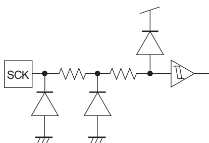
Fig.59 SCK input equivalent circuit
