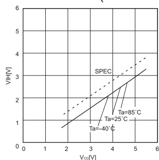
Fig.6 "H" input voltage V_{IH}(C\bar{S}, SCK, SI, \overline{HOLD}, \overline{WP})
