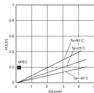
Fig.8 "L" output voltage V_{OL}-I_{OL}(V_{CC}=1.8V)
