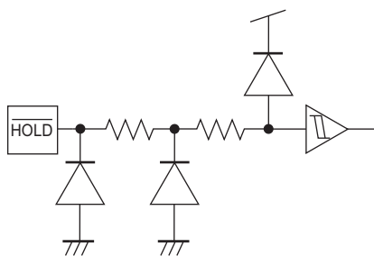
Fig.61 \overline{\text{HOLD}} input equivalent circuit
