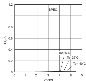
Fig.12 Input leak current I_{IL}(CS,SCK,SI,WP,HOLD)
