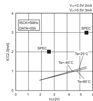
Fig.14 Current consumption at WRITE operation ICC1,2,3(WRITE,PAGE WRITE,WRSR,fSCK=5MHz) BR25L010-W,BR25L020-W,BR25L040-W
