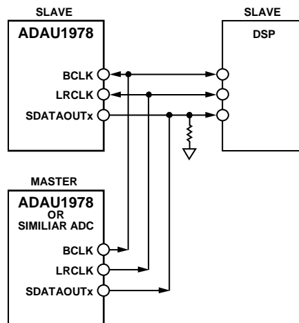
Figure 31. Serial Port Connection Option 4—TDM Mode, Second ADC Master
