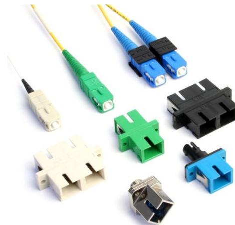
Multiple Options on SC Adapters
