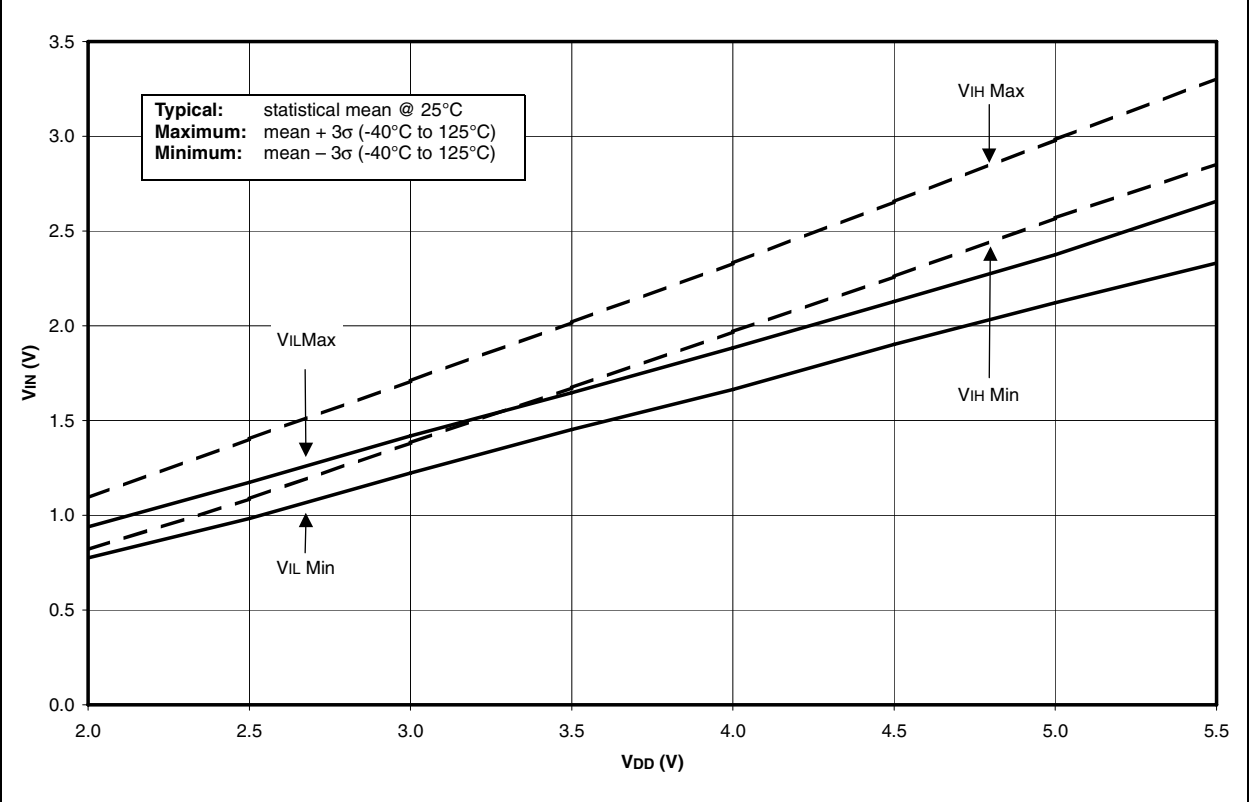
FIGURE 23-27: MINIMUM AND MAXIMUM VIN vs. VDD (I 2 C INPUT, -40°C TO +125°C)
