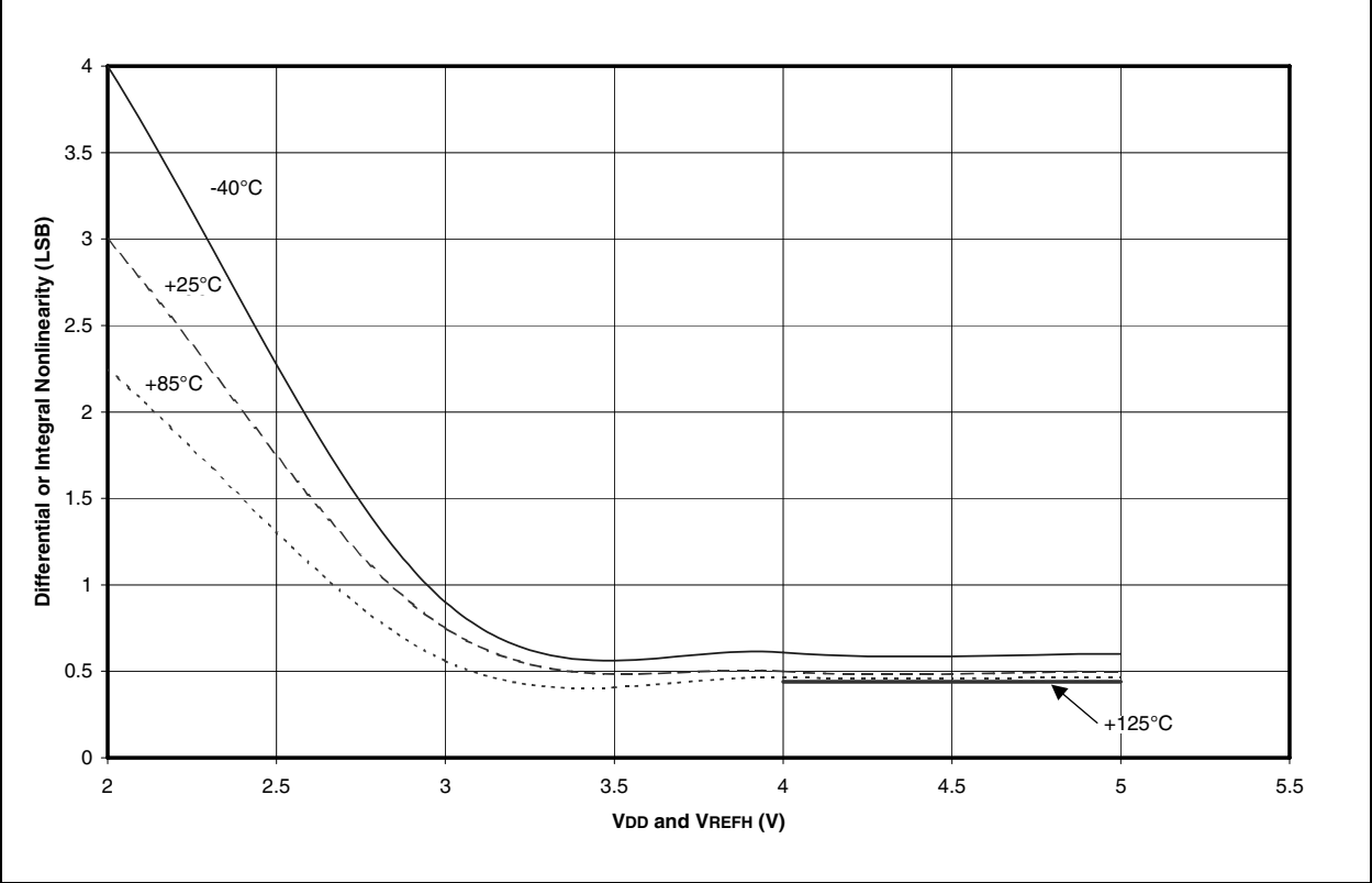
FIGURE 23-28: A/D NON-LINEARITY vs. VREFH ( V_{DD} = V_{REFH} , -40°C TO +125°C)
