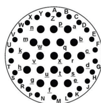
25-43 - 25-43 No. of Contacts 23 #20, 20 #16 Service Ratings I
