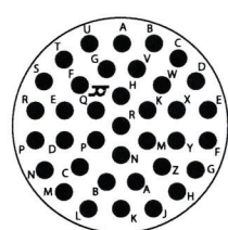
25-37 - 25-37*• No. of Contacts 37 #16 Service Ratings II I
