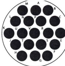
25-19 - 25-19 No. of Contacts 19 #12 Service Ratings I
